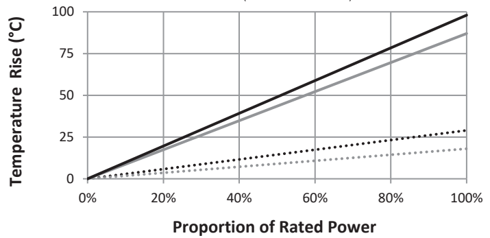
2817 Typical Temperature Rise (mounted on FR4 board)
