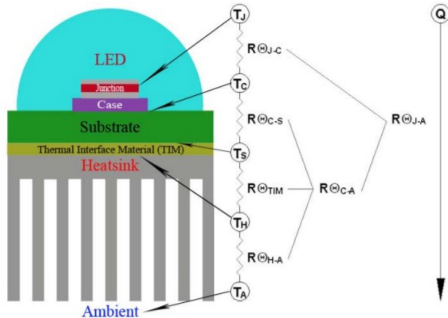
Figure 1 - Thermal Model for Single-Component Assembly
