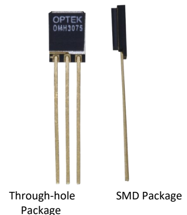
OMH3075 Bipolar Hall Effect Sensor
