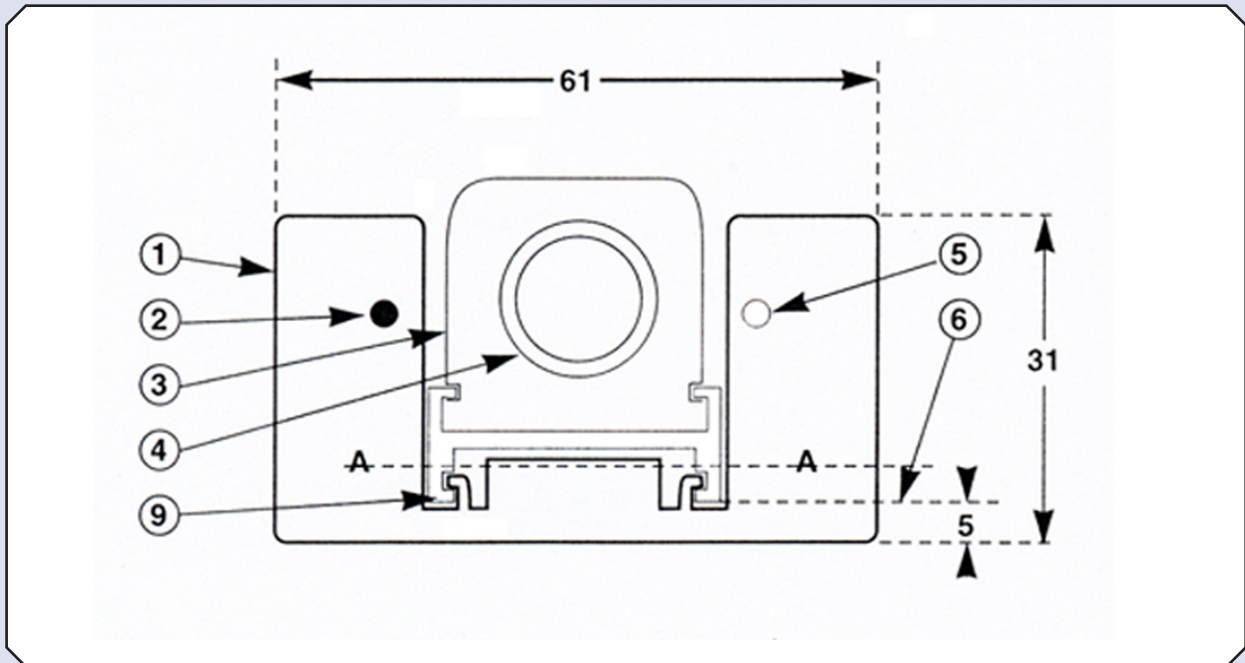
Figure 1 - Plan view of GIR sensor fitted to NG/LG flowmeter frame.
