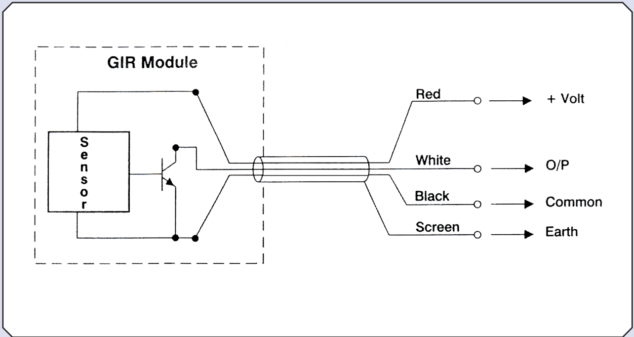
Figure 4 - Electrical Connections
