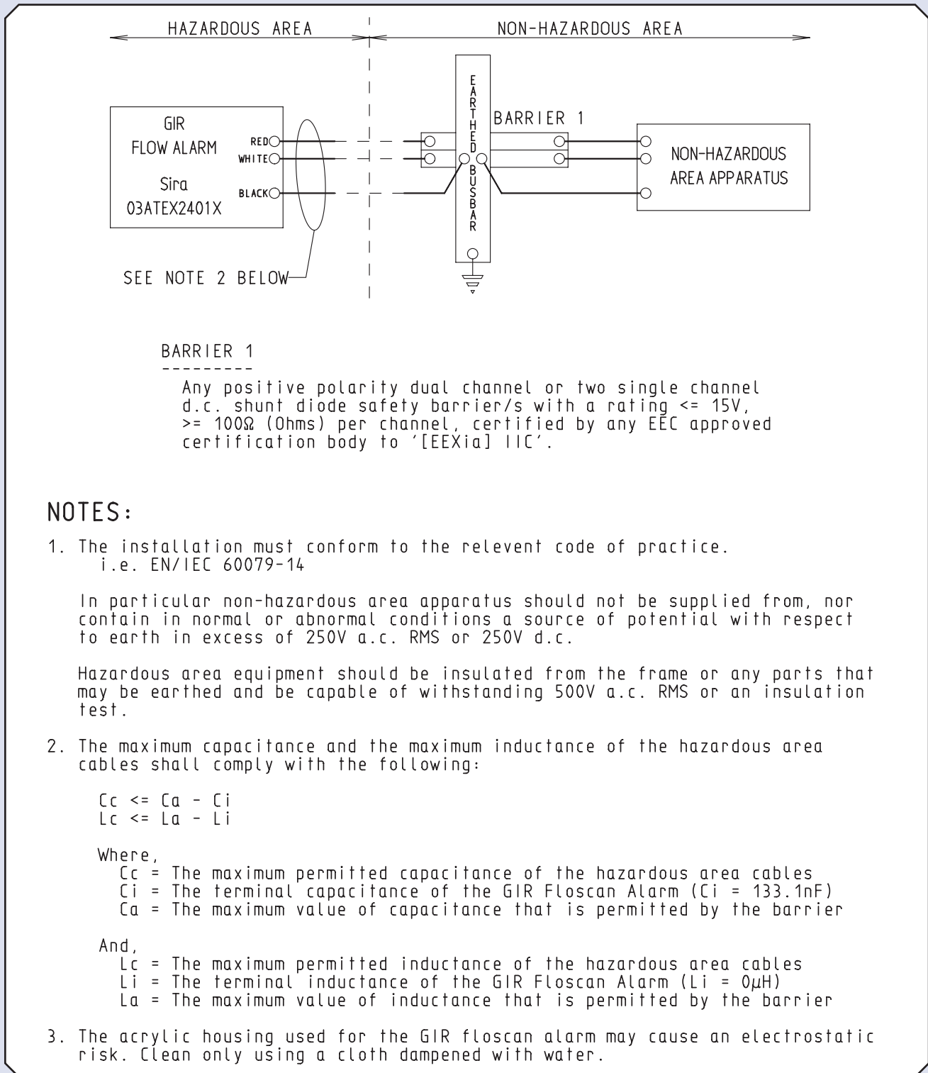
Figure 6 - Intrinsically Safe Installation (2-W142)
