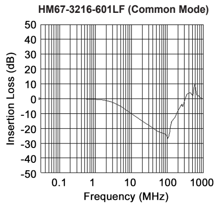
(B) Insertion Loss vs. Frequency Graphs (Cont'd)
