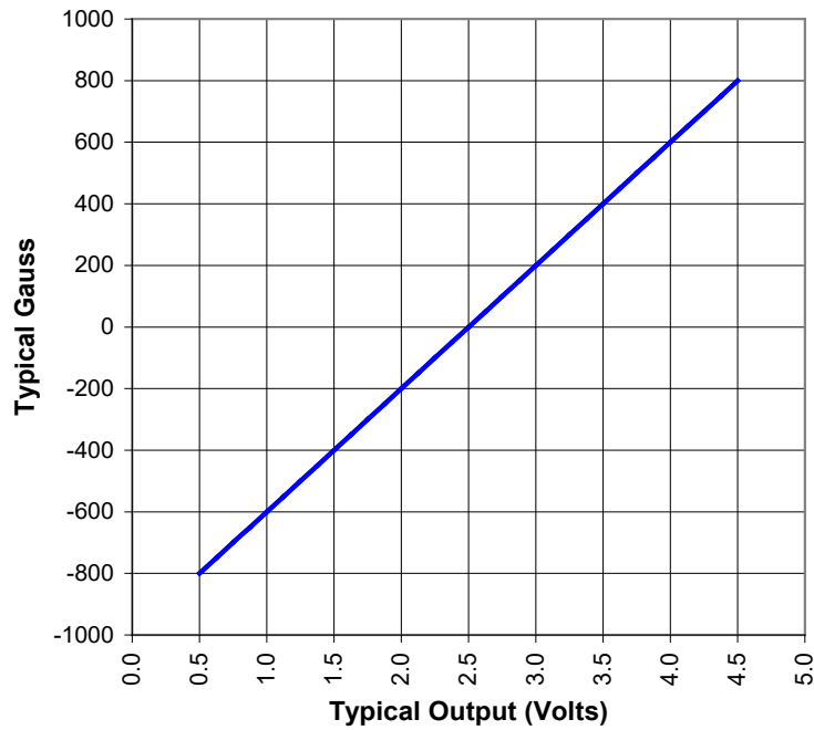
Output vs Gauss
