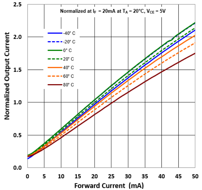
Output Current vs Forward Current vs Temp
