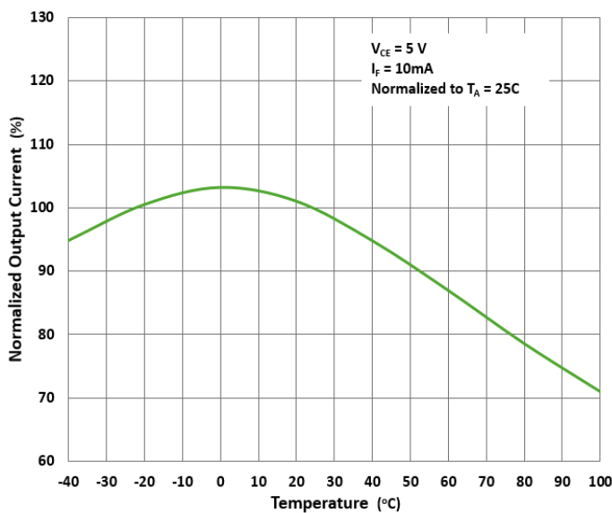
Output Current vs Temperature
