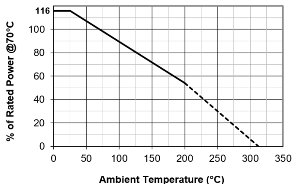
Temperature Derating
