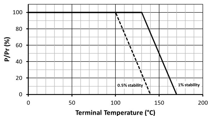
Temperature Derating
