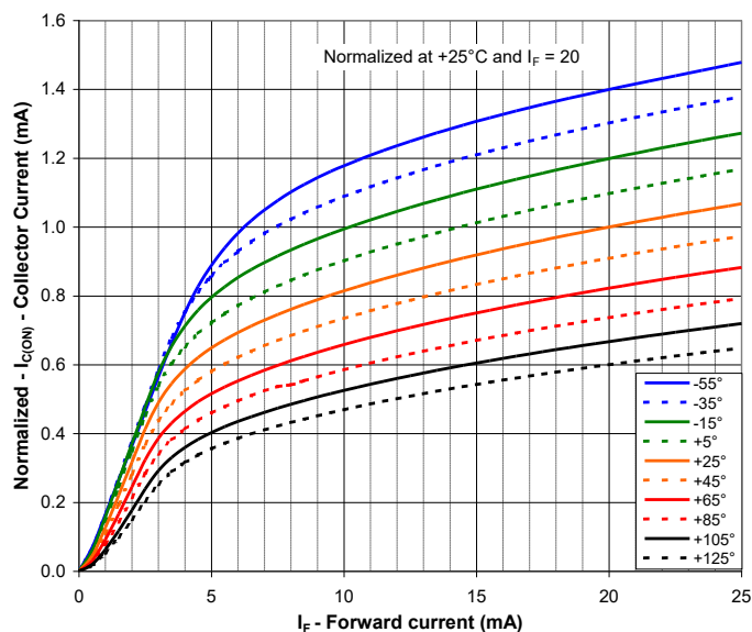
Collector Current vs Forward Current vs Temperature
