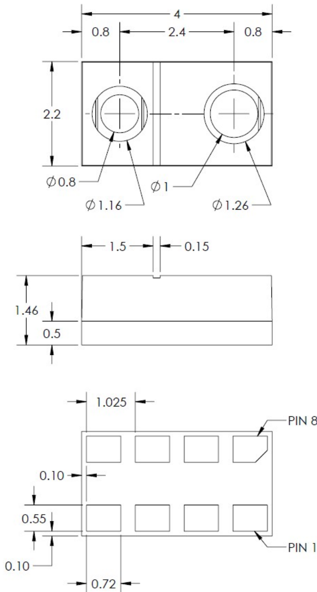
Package Outline, Pinout, and Function Table
