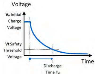
Figure 3 Exponential discharge
