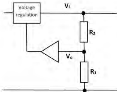
Figure 8 Voltage Divider
